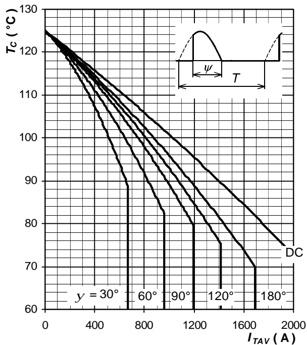
Fig. 10 Max. case temperature vs. aver. on-state current, sine waveform, f = 50 Hz, T = 1/f
