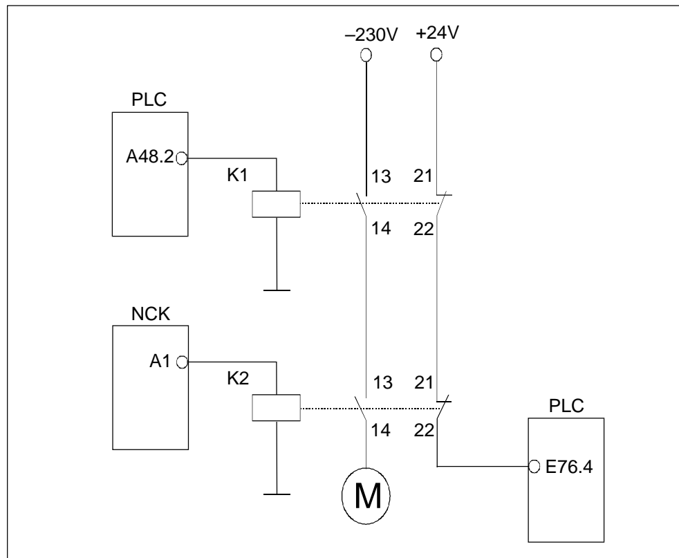
Fig. 10-8 Circuit diagram
