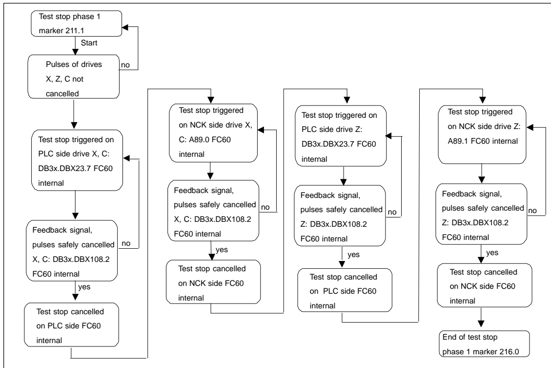
Fig. 10-12 Function diagram
