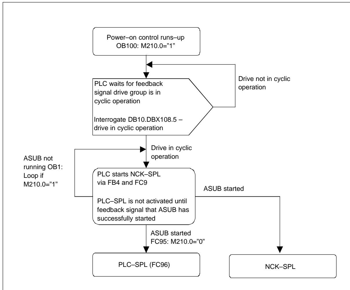
Fig. 10-4 Flowchart
